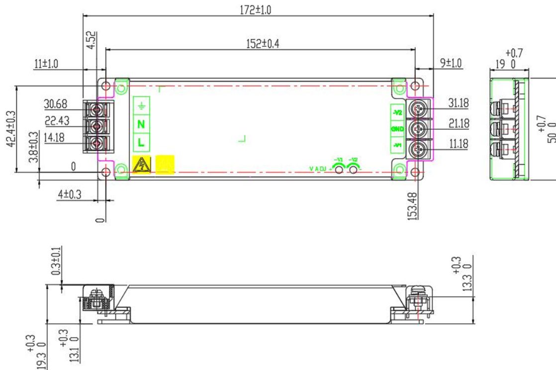
Definition and Installation Notes for Input Terminal and Output Terminal
